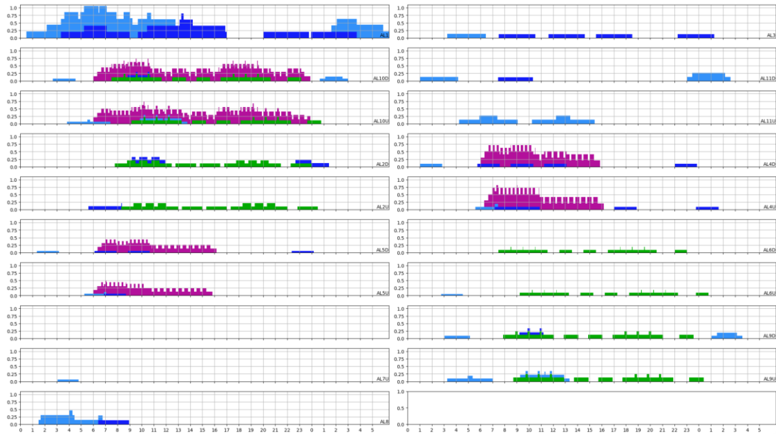
Figure 12 A capacity model when a TCR is introduced along line section AL2.
