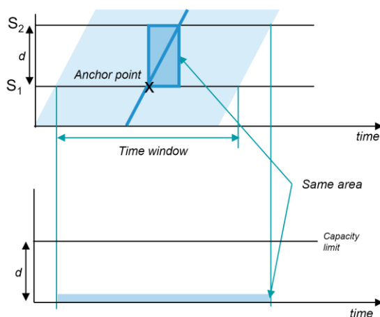
Figure 9. The relation between a prognosticated train path and a transportation path (bandwidth).
