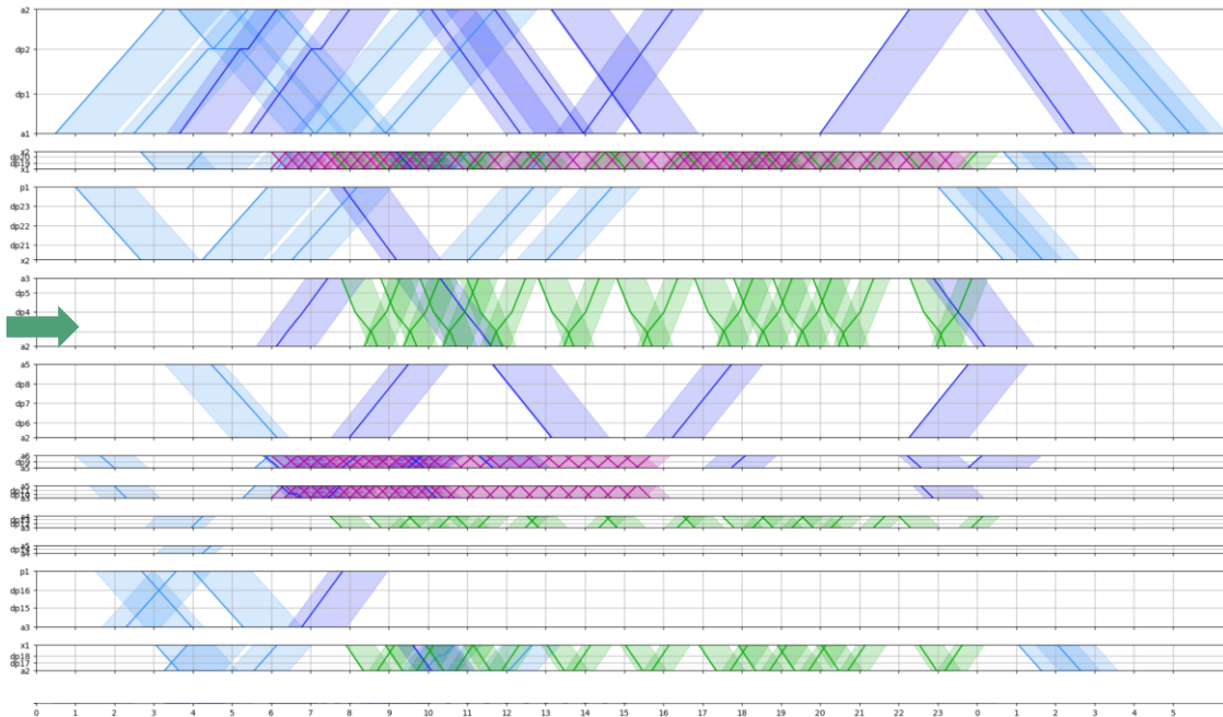
Figure 13 Detailed schedule (ATT) of a scenario with a TCR between operational points DP3 and DP4 leading to single track operation and reduced speed.
