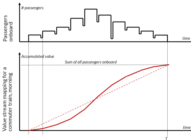
Figure 3 Number of passengers onboard as a function of time, and the corresponding value stream mapping
