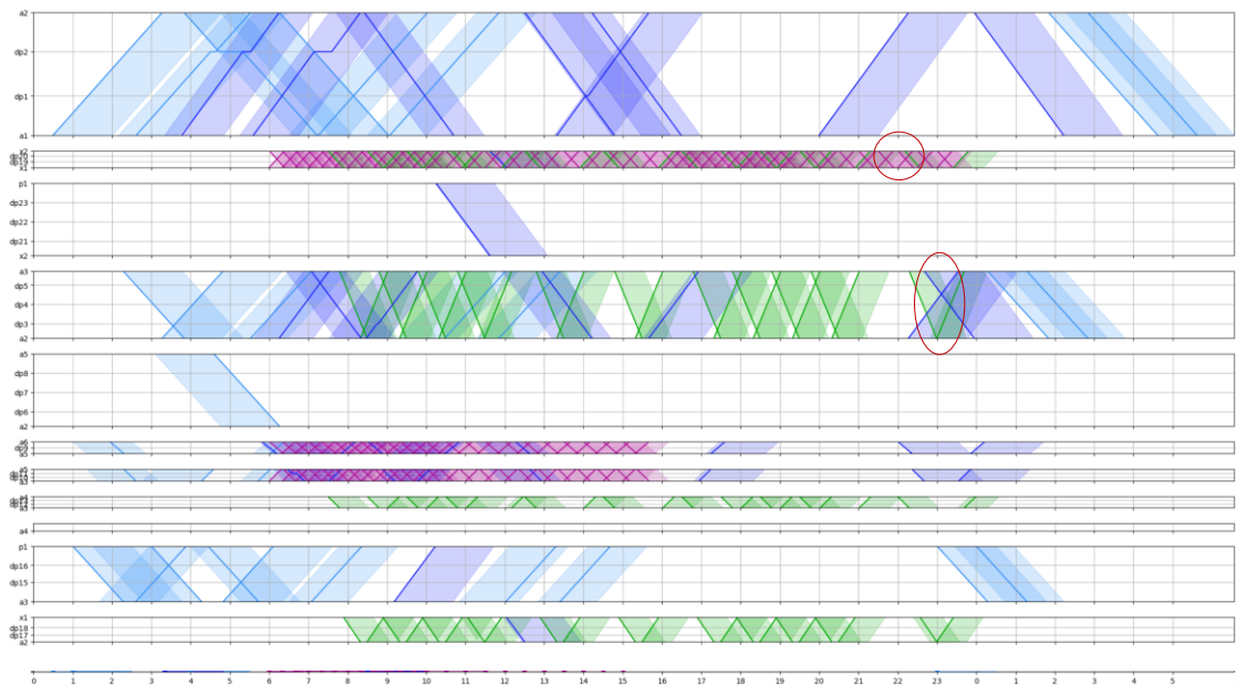
Figure 17 Schedule using the national cost parameters
