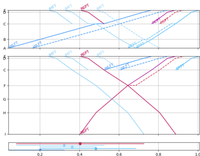
Figure 7. Plotting the two schedules in the same graph.
